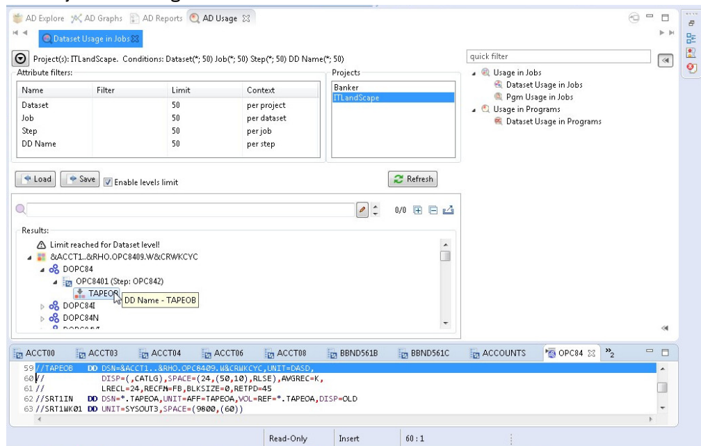
Figure 37. Dataset Usage in Jobs
